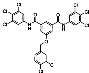
Compound # 32
